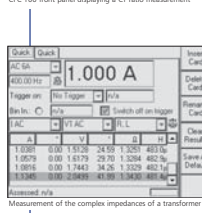
Measurement of the complex impedances of a transformer
