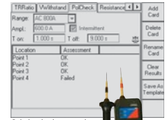
Polarity check test card
